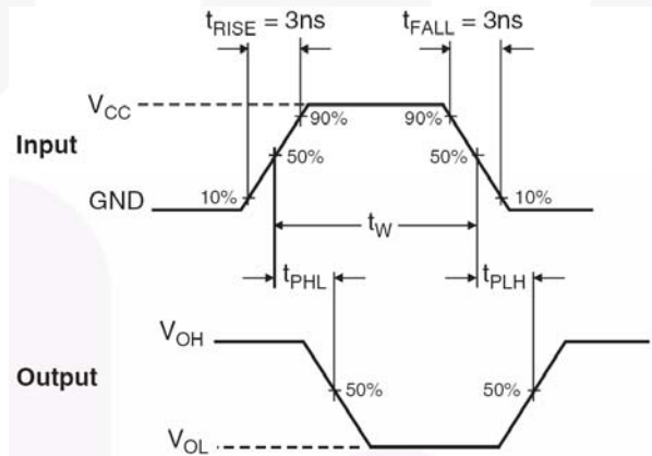
Figure 6. AC Waveforms
