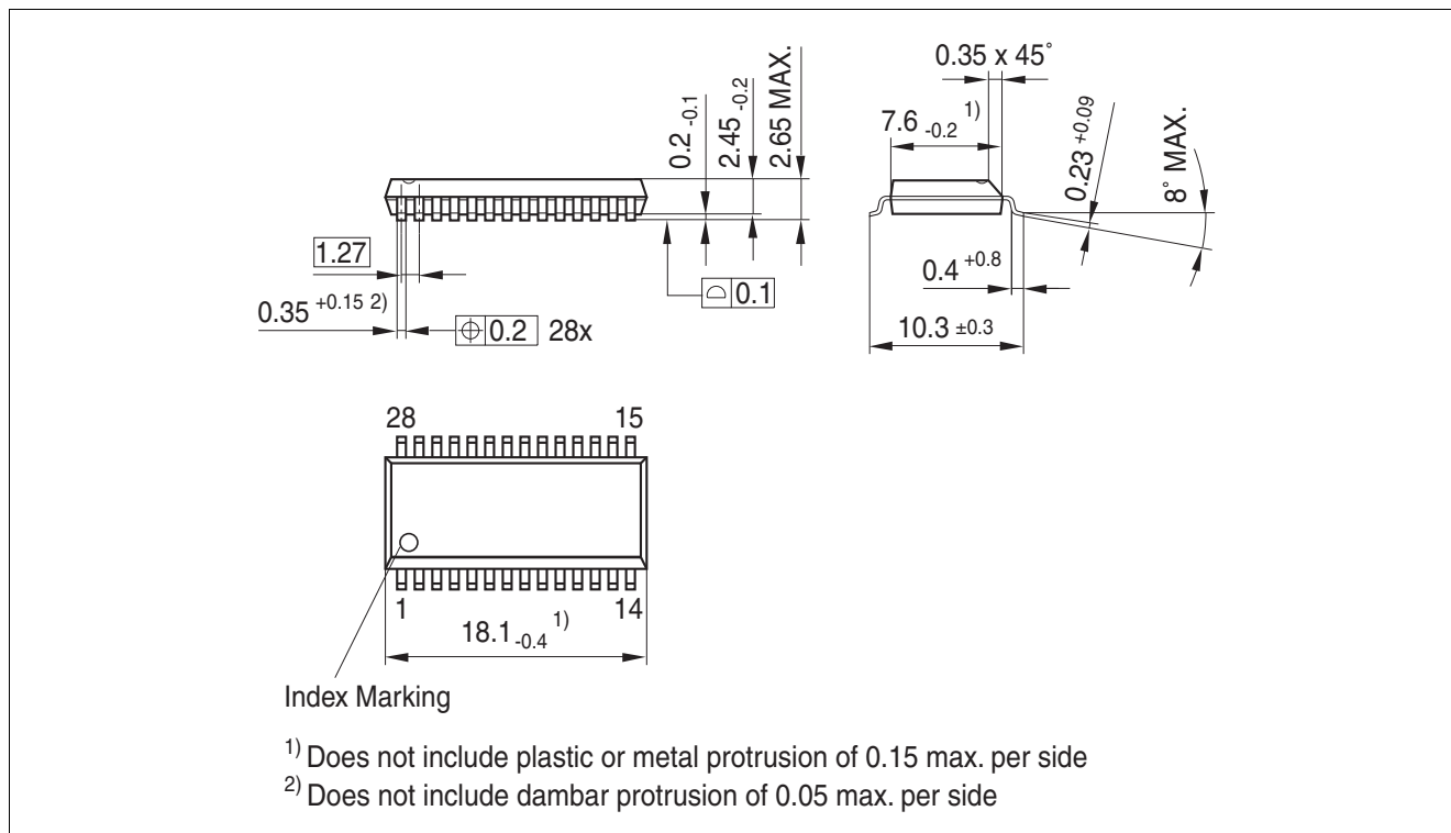
Figure 4 PG-DSO-28
