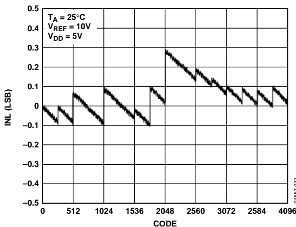
Figure 8. INL vs. Code (12-Bit DAC)
