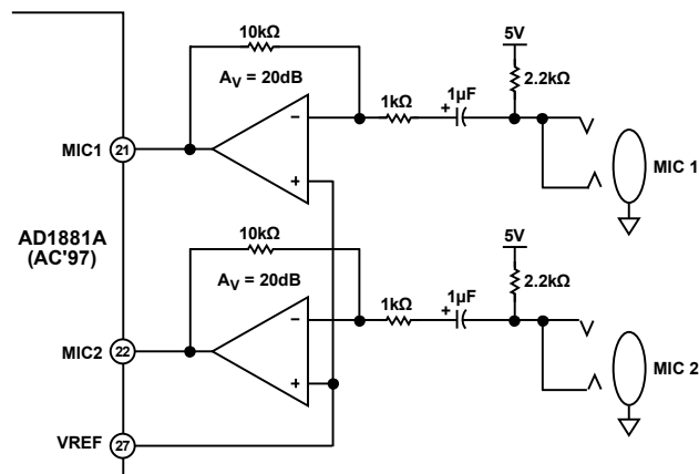
Figure 32. Microphone Preamplifier
