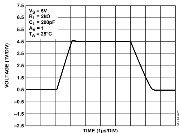
Figure 7. Large Signal Transient Response, V_S = 5V
