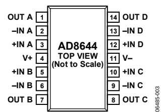
Figure 3. 14-Lead Narrow Body SOIC (R-14)
