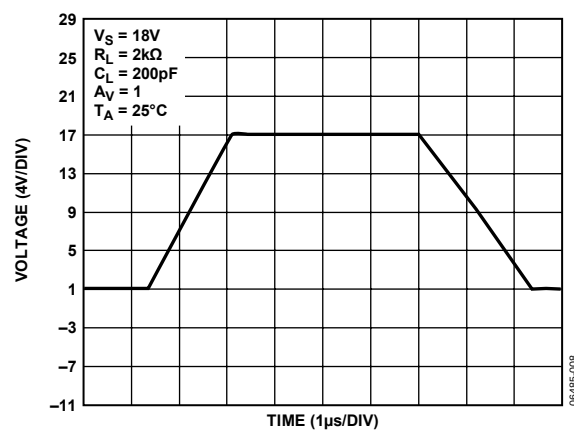
Figure 8. Large Signal Transient Response, V_S = 18V
