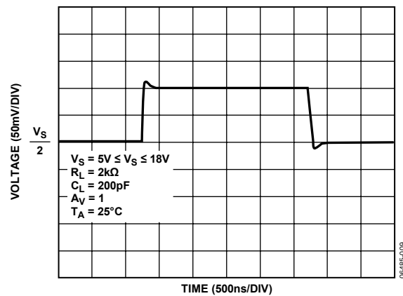
Figure 9. Small Signal Transient Response
