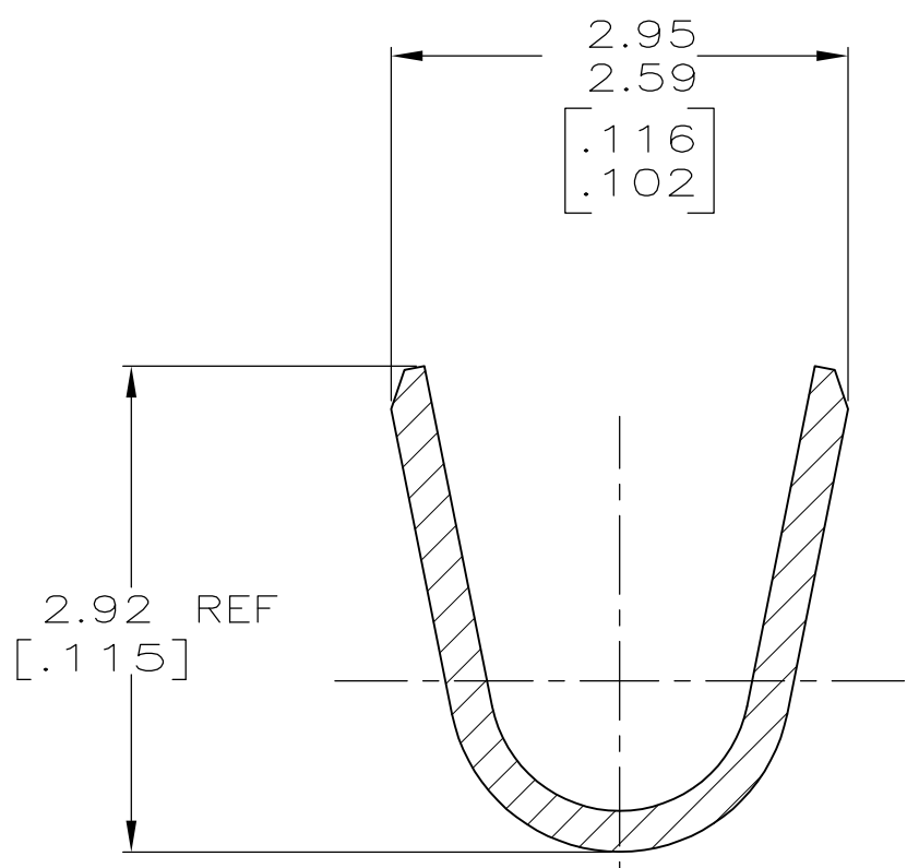
SECTION B—B SCALE 20:1
