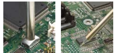
MFR-2200 Series Hand-pieces A. MFR-H4-TW Precision Tweezers B. MFR-H1-SC Soldering Cartridge C. MFR-H2-ST Soldering Tip
