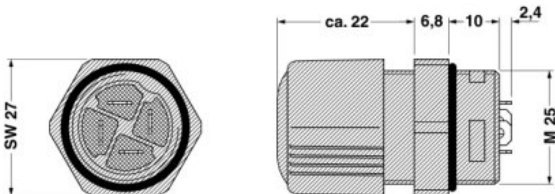
Dimensioned drawing
