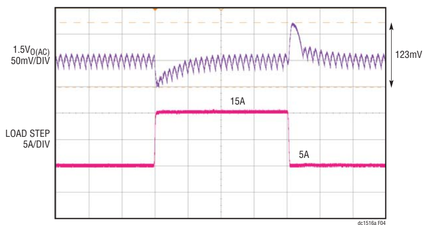
Figure 4. Load Step Response of the DC1516A-A (DCR SENSE) at V_{IN} = 12V . C_{OUT} = 2 \times \text{Sanyo 2R5TPE330M9} \parallel 2 \times 100\mu F \text{ X5R } 6.3V \ 1206 , L = 0.56\mu H , f_{SW} = 300kHz
