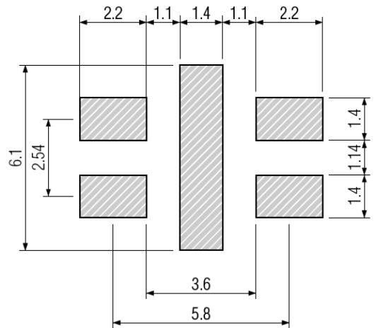
Figure 3) Land Pattern
