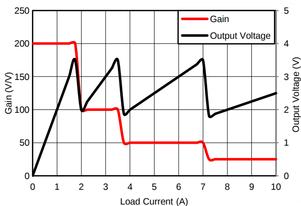
Figure 40. Microcontroller-Configured Gain Selection Response
