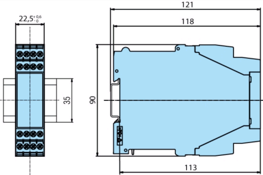
KNE3-YS - Screw terminals
