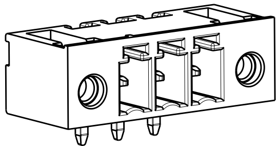
284541-3 AS SHOWN
