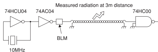
Testing Circuit
