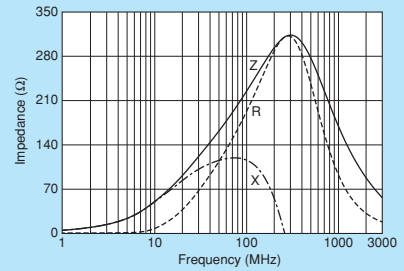
BLM15PX221SN1
