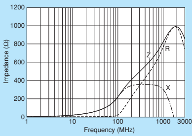
BLM15HB221SN1
