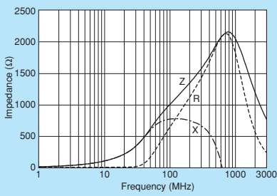
BLM15HD102SN1
