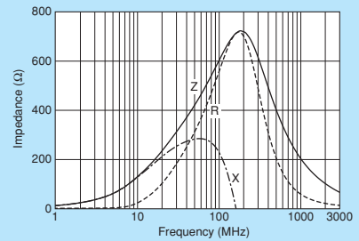
BLM15PX601SN1
