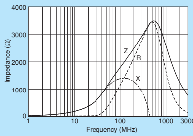
BLM15HD182SN1
