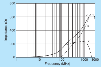
BLM15HB121SN1
