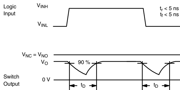
Figure 3. Break-Before-Make (DG419L)
