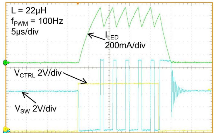
Figure 37. 0.2% PWM Duty Cycle at 100Hz PWM Frequency and 22μH Inductance
