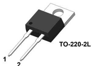
1. Cathode 2. Anode
