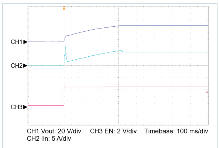
Figure 14 — Startup from EN, V_{IN} = 30\text{ V} , C_{OUT\_EXT} = 10000\text{ }\mu\text{F} , R_{LOAD} = 4.828\text{ }\Omega
