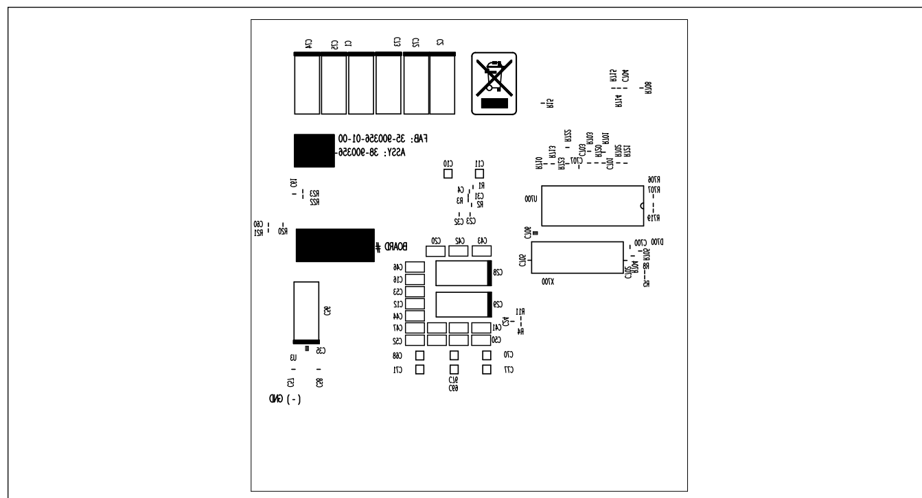
Bottom Silkscreen
