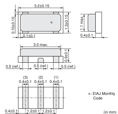
CSTCE_V_C 14.00-20.00MHz
