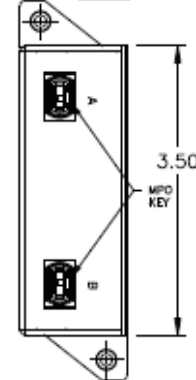
MOUNTING STYLE H1 REAR STYLE FLAT LC QUAD
