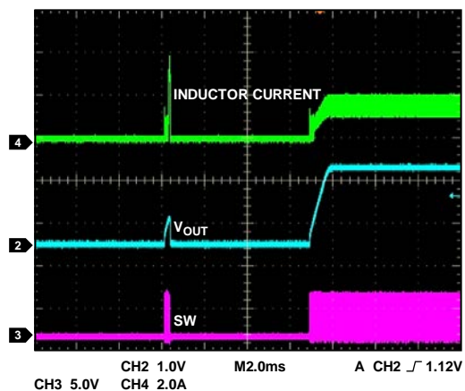
Figure 57. Exit Hiccup Mode, Channel 2 V_{OUT} = 1.8 V, f_{SW} = 600 kHz
