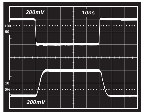
TPC 24. Inverter Small Signal Pulse Response; V_S = \pm 5V , C_F = 1pF , R_L = 150W
