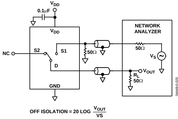
Figure 21. Off Isolation
