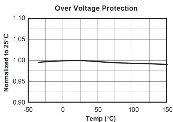
Figure 11. Over-Voltage Protection
