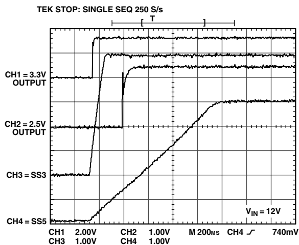
Figure 13. Soft-Start Sequencing
