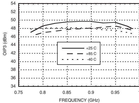
Output IP3 vs. Temperature @ 900 MHz
