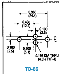
TO-66
