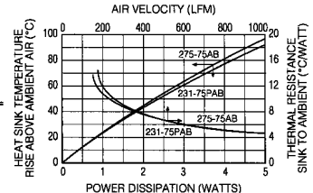
NATURAL AND FORCED CONVECTION CHARACTERISTICS
