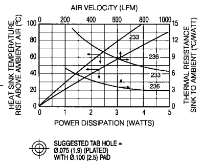
NATURAL AND FORCED CONVECTION CHARACTERISTICS
