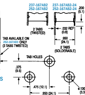
237 AND 252 SERIES Dimensions: in. (mm)
