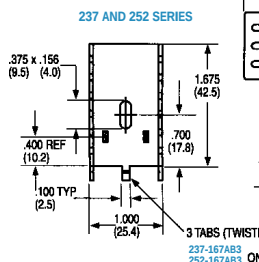
237 AND 252 SERIES Dimensions: in. (mm)
