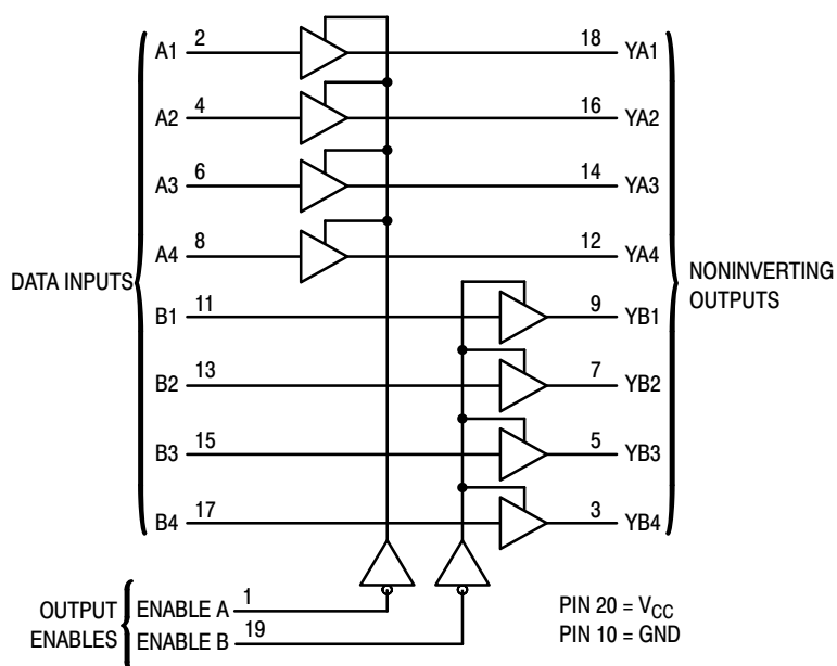
Figure 1. Logic Diagram
