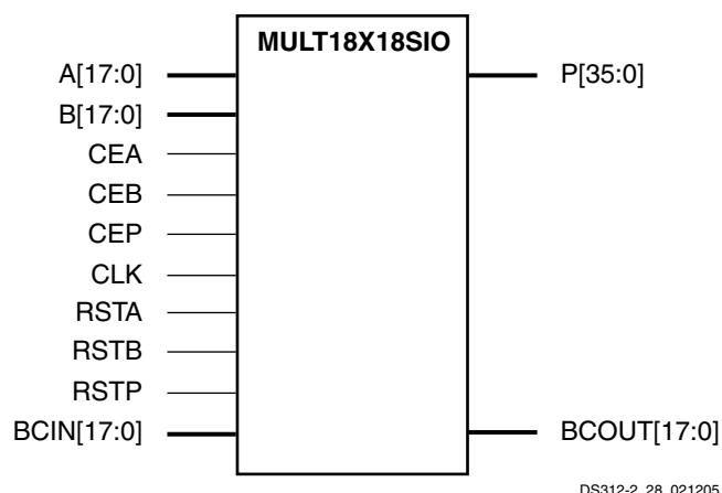
Figure 37: MULT18X18SIO Primitive
