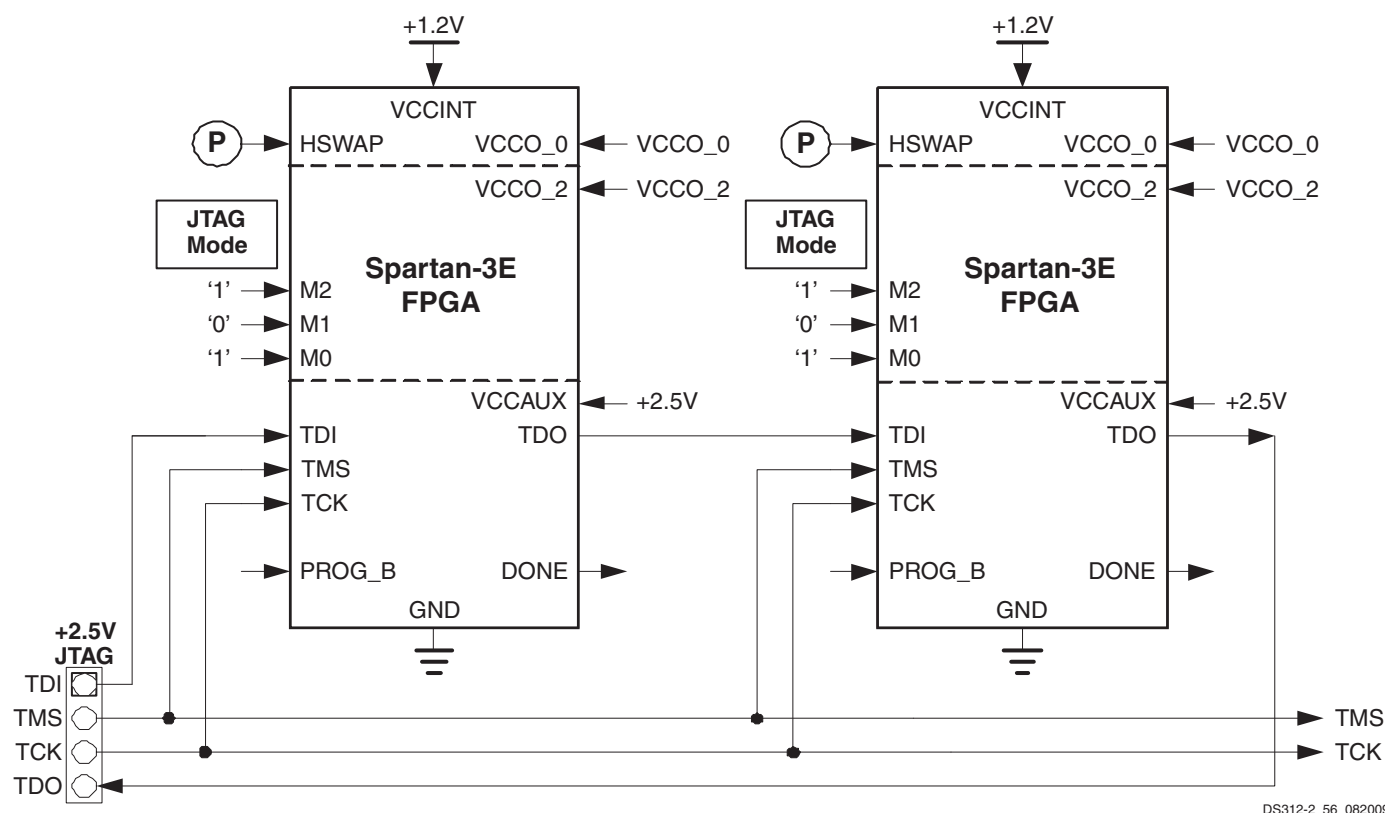
Figure 65: JTAG Configuration Mode
