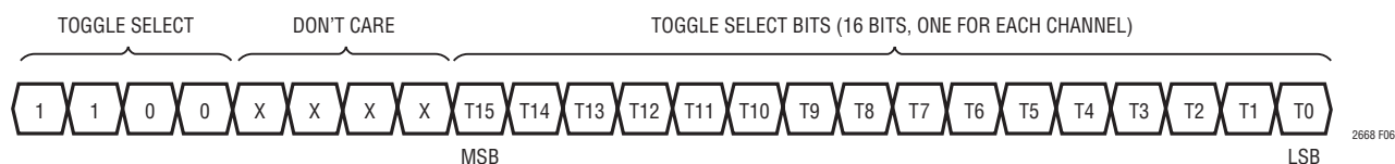
Figure 6. Toggle Select Syntax
