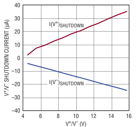
V^+/V^- Shutdown Current vs Symmetric Supplies
