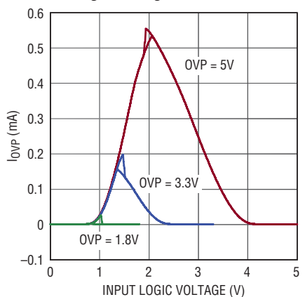
I_{OVP} Supply Current vs Logic Voltage
