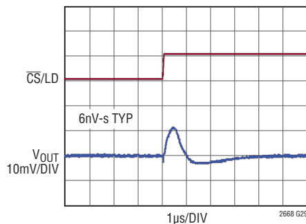
DAC-to-DAC Crosstalk
