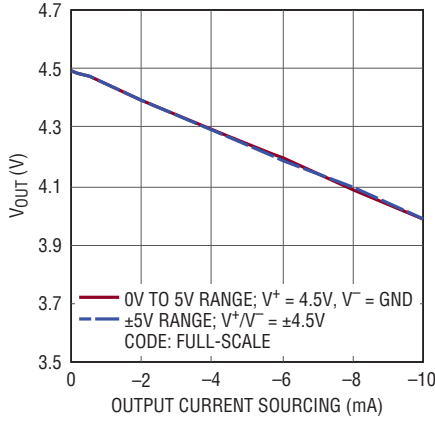
Headroom to V^+ Rail vs Output Current
