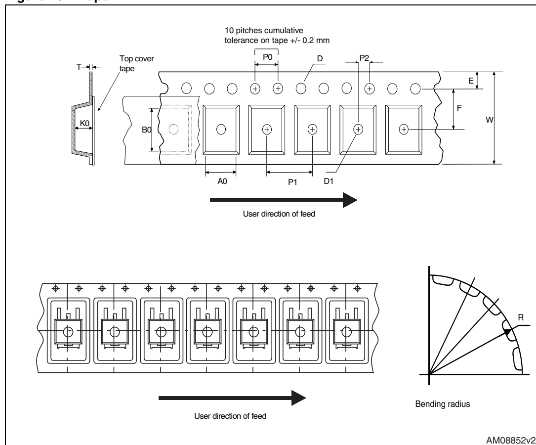
Figure 28. Tape
