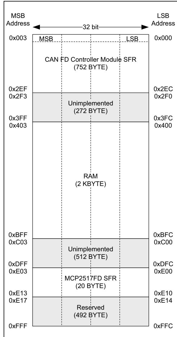
FIGURE 3-1: MEMORY MAP
