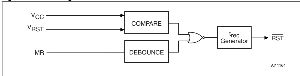
Figure 3. Block diagram
