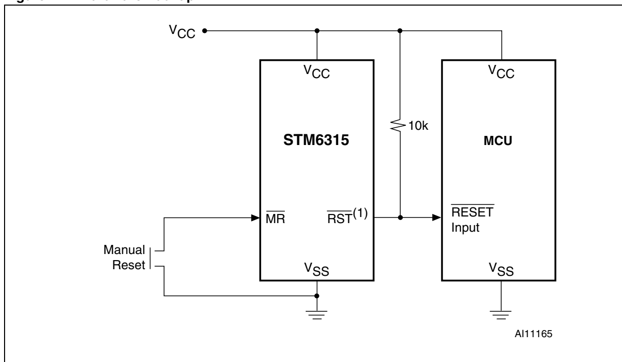
Figure 4. Hardware hookup
