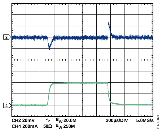
Figure 25. Channel 4 Load Transient, V_{OUT} = 3.3\text{ V} , FPWM Mode
