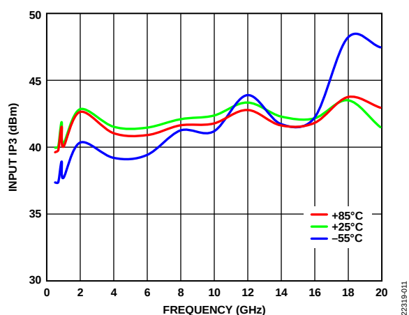
Figure 11. Input IP3 vs. Frequency over Temperature, V_{CTL} = -5\text{ V}
