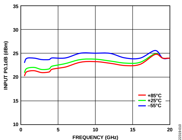
Figure 10. Input P0.1dB vs. Frequency over Temperature, V_{CTL} = -5\text{ V}
