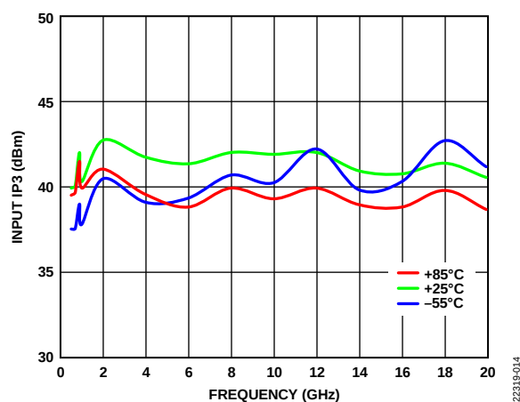
Figure 14. Input IP3 vs. Frequency over Temperature, V_{CTL} = -3\text{ V}
