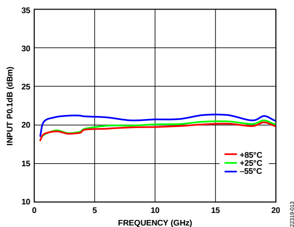
Figure 13. Input P0.1dB vs. Frequency over Temperature, V_{CTL} = -3\text{ V}
