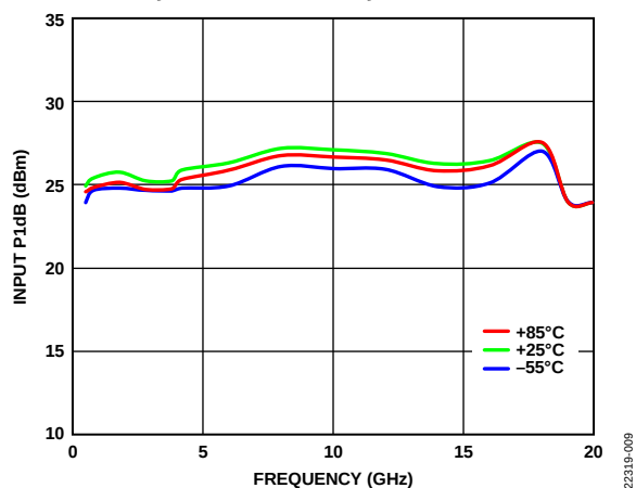
Figure 9. Input P1dB vs. Frequency over Temperature, V_{CTL} = -5\text{ V}
