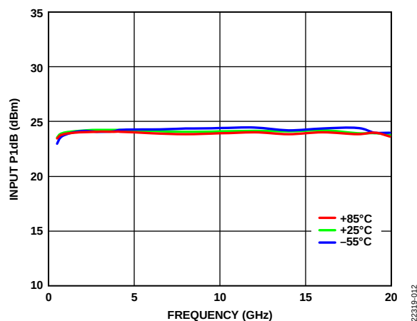
Figure 12. Input P1dB vs. Frequency over Temperature, V_{CTL} = -3\text{ V}
