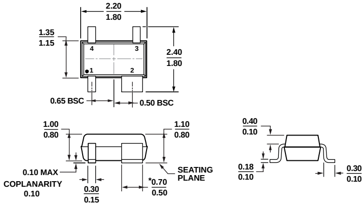
*PACKAGE OUTLINE CORRESPONDS IN FULL TO EIAJ SC82 EXCEPT FOR WIDTH OF PIN 2 AS SHOWN. Figure 14. 4-Lead Thin Shrink Small Outline Transistor Package [SC70] (KS-4) Dimensions shown in millimeters
