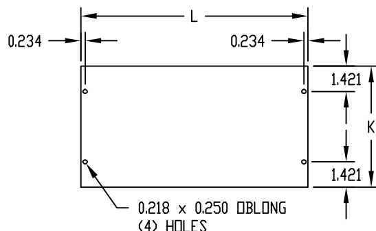
REAR PANEL
