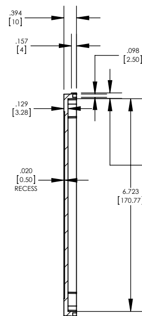
SECTION B-B
