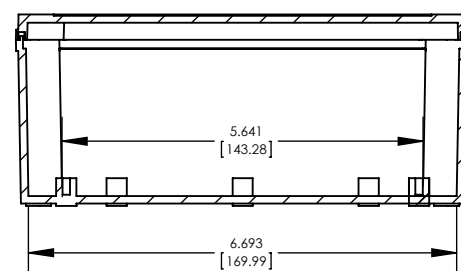
SECTION E-E
