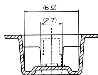
SECT. C-C
