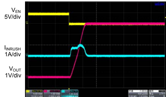
Time 500µs/div
