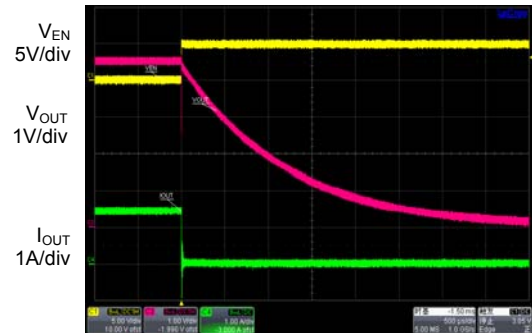
Time 500µs/div
