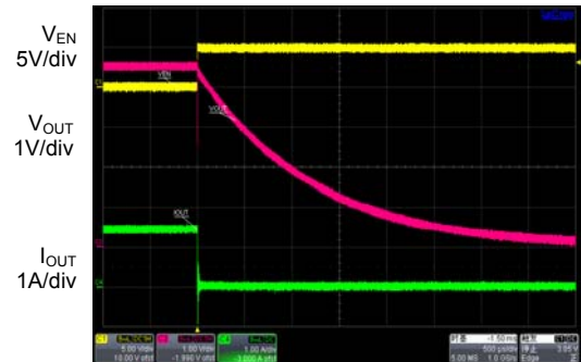
Time 500µs/div
