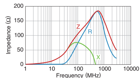
MPZ1608Y101BTA00
