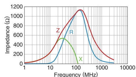
MPZ1608S102ATA00
