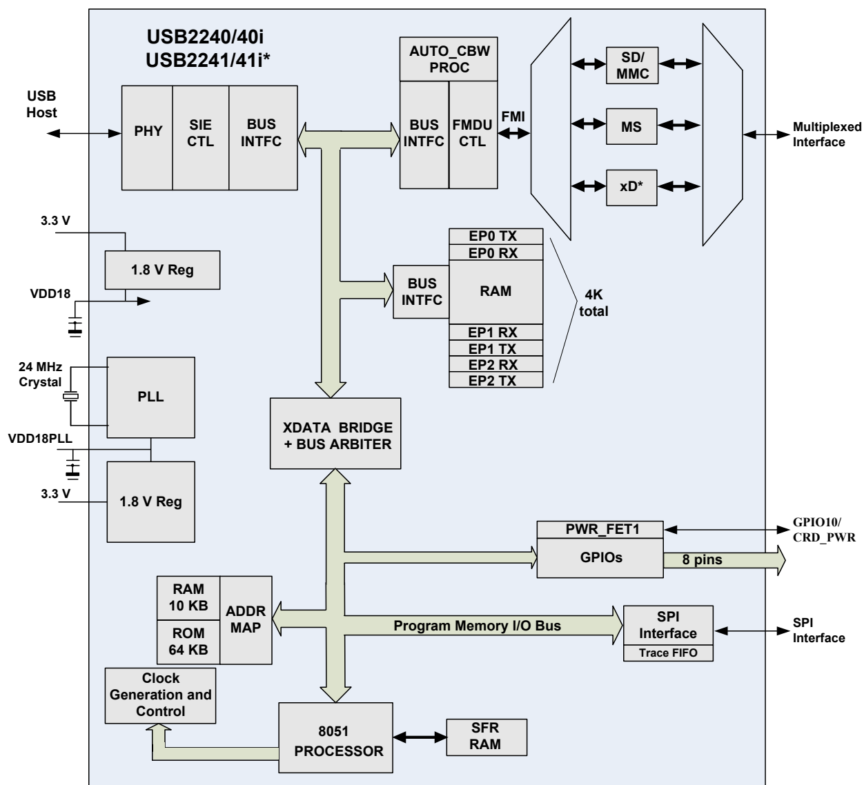
Figure 3.1 USB2240/40i/41/41i Block Diagram
